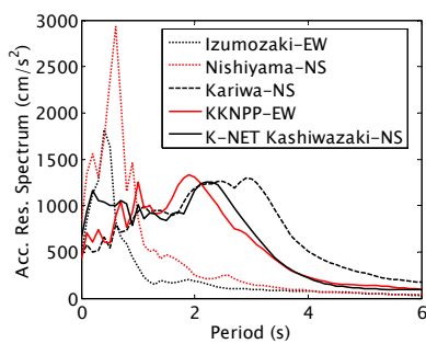
Figure 3 Response spectrum of acceleration.
