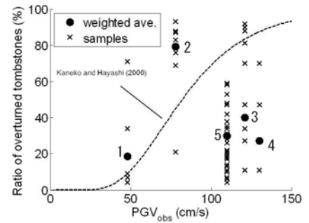
Figure 5 PGV obs and ratio of the overturned tombstones.
