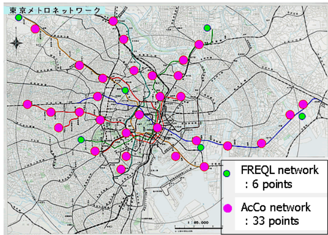
Fig.1 The seismometer system of Tokyo Metro
