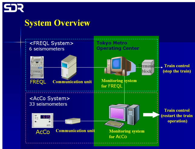
Fig.2 The system overview of Tokyo Metro
