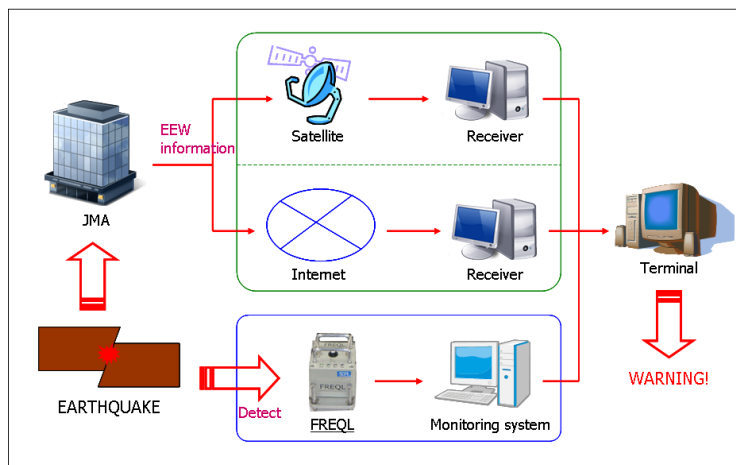
Fig.3 The system overview of Onagawa nuclear power station
